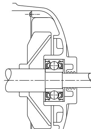
Fig. 174. W-PP type typical mounting.
