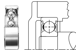
Fig. 164. Two shields, suffix DD.
