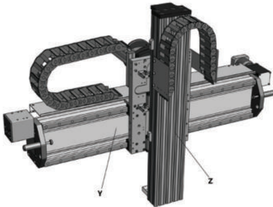
Figure 7.8 ___ Standard combination AXS – Lifting Axis with AXS – Gantry Axis with toothed belt drive
