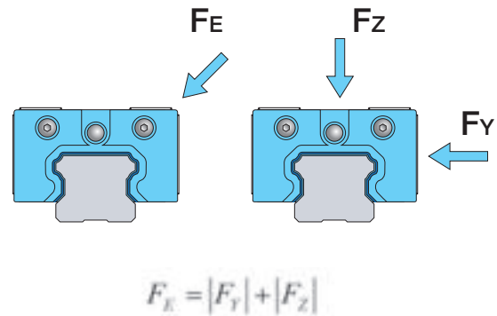
Figure 2.2 ___ Equivalent load
