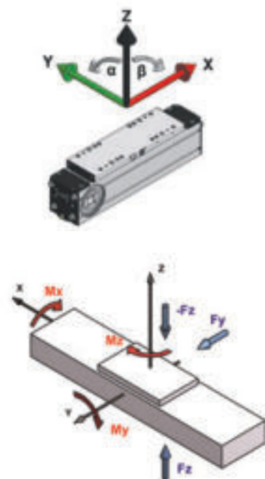
Figure 2.1 ___ Coordinate system
